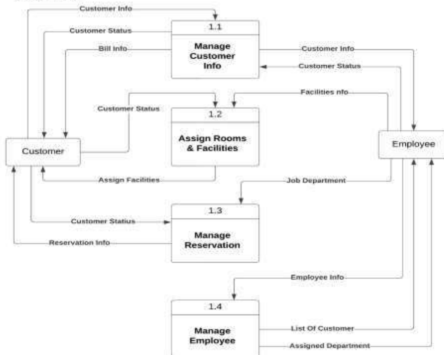
Level 1 DFD :-
